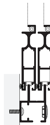
Frame profile
