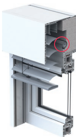
In the top-mounted box
