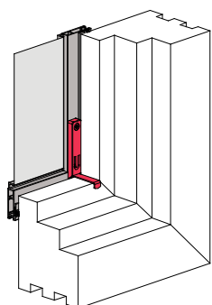
Suspension bracket spring-mounted
