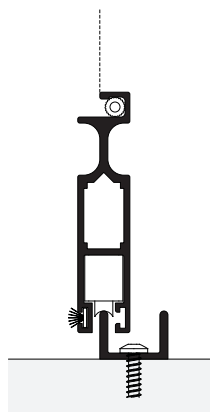
U-profile
