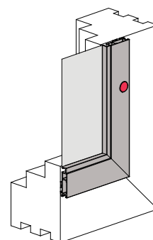
Installation with screws
