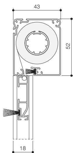
Square design
